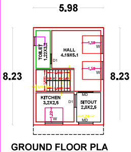
GROUND FLOOR PLA
