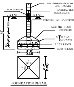
FOUNDATION DETAIL
