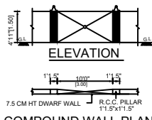
COMPOUND WALL PLAN
