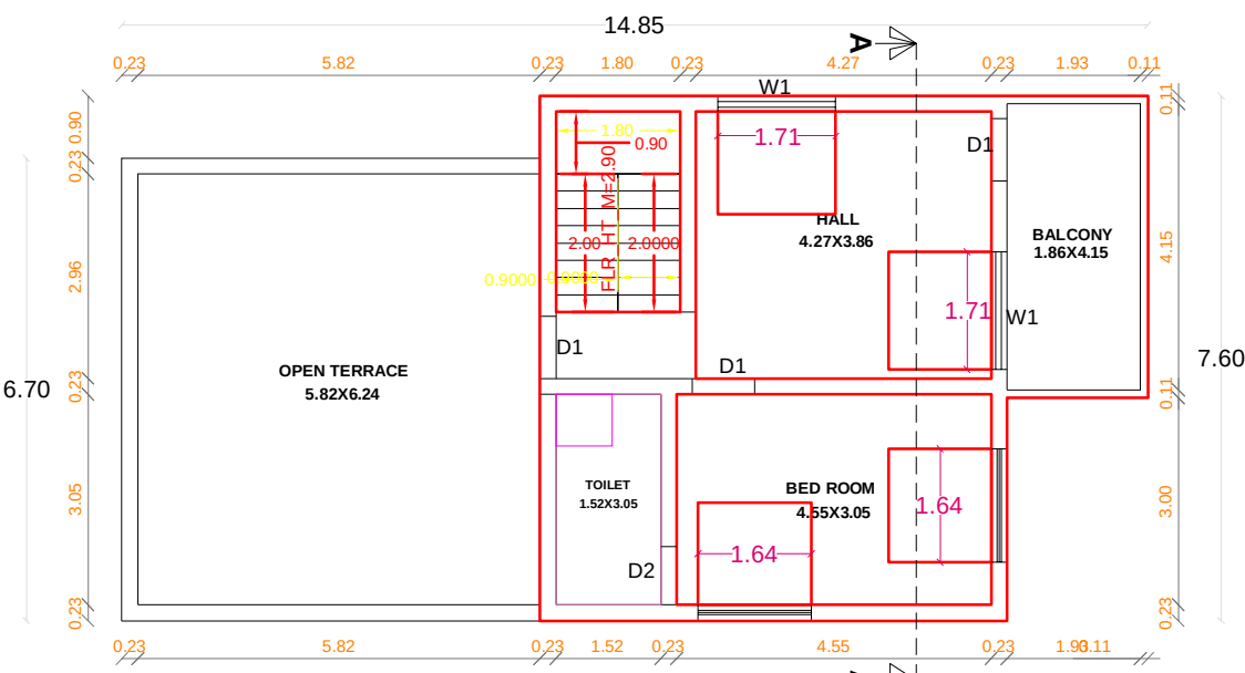
FIRST FLOOR PLAN PROPOSED
