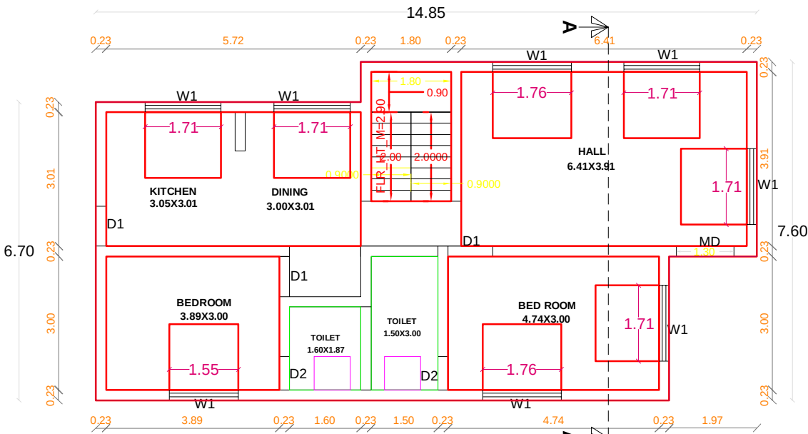
GROUND FLOOR PLAN PROPOSED
