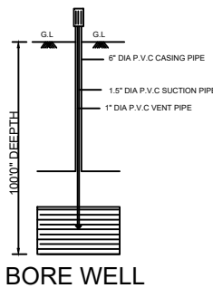
BORE WELL
