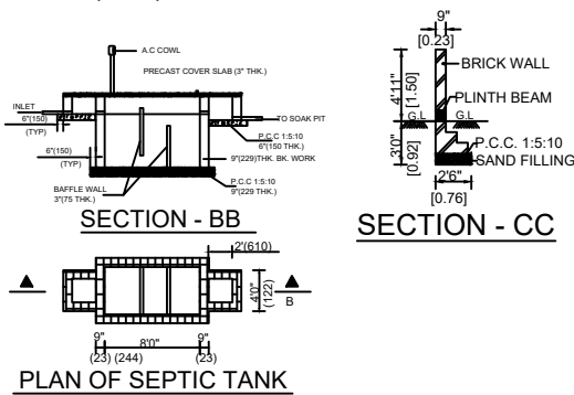
FOUNDATION DETAIL
