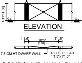
COMPOUND WALL PLAN
