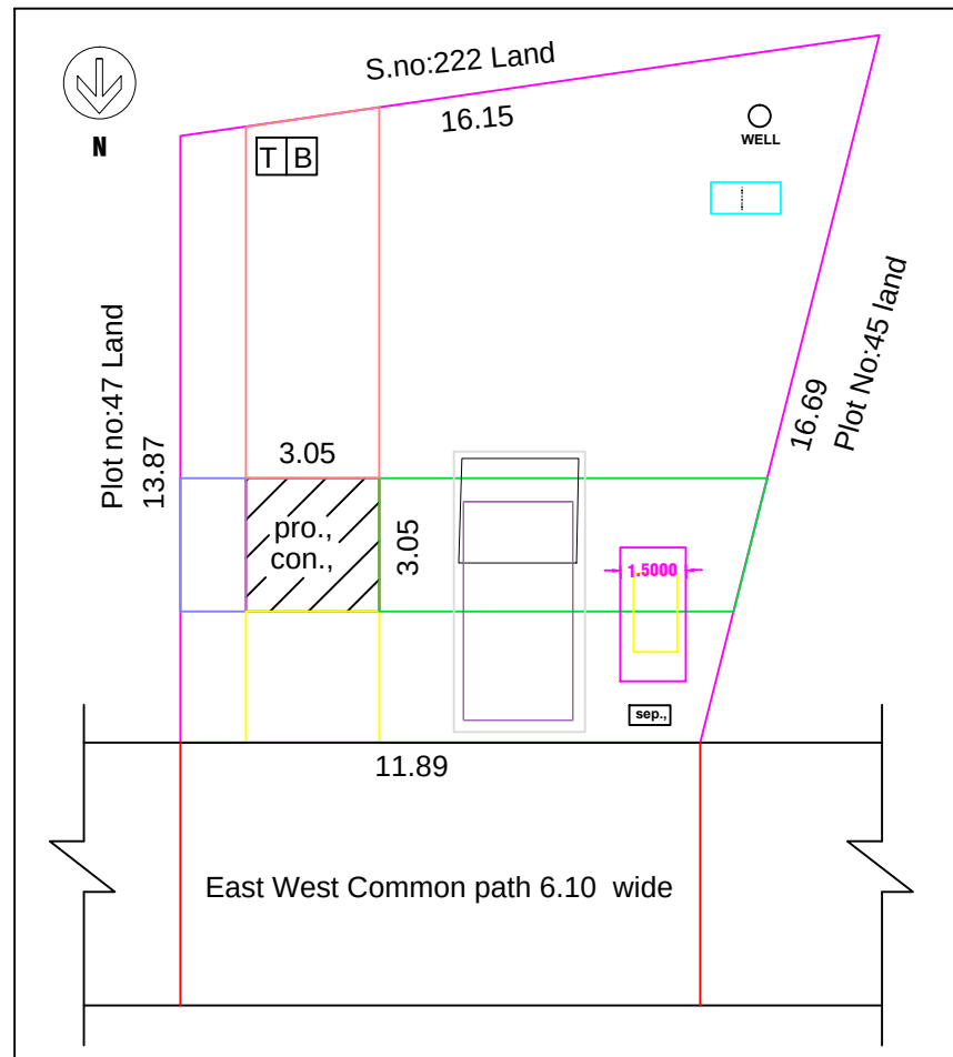
SITE PLAN & KEY PLAN
