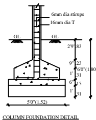
COLUMN FOUNDATION DETAIL
