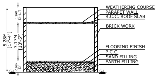
SECTION AN AA
