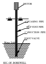
SEC. OF BOREWELL
