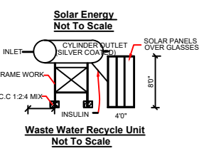
Solar Hot Water System Detail
