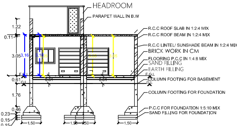
SECTION ON-AA
