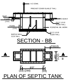
SECTION - BB PLAN OF SEPTIC TANK
