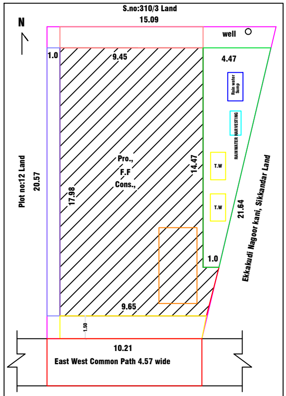
SITE PLAN & KEY PLAN (1:100)
