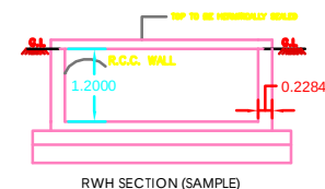
RWHP_CAPACITY_L=2000LTRS
