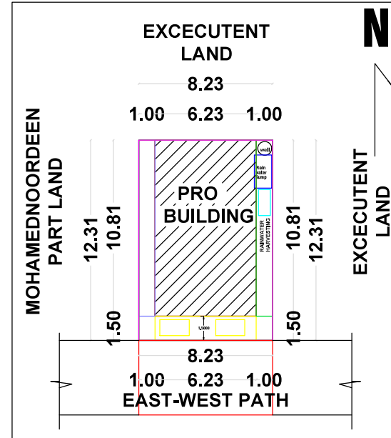
SITE PLAN & KEY PLAN (1:100)
