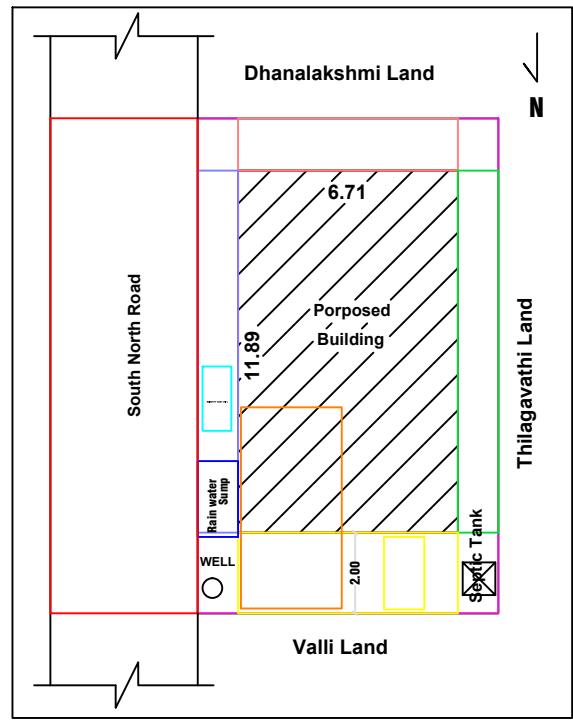
SITE PLAN CUM KEYPLAN
