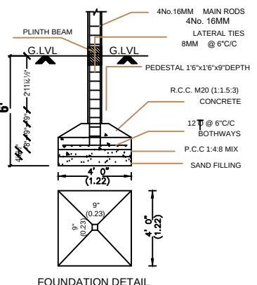
FOUNDATION DETAIL
