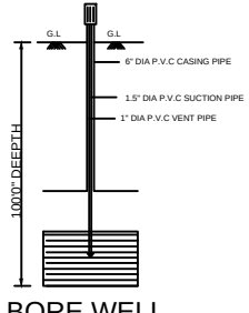
BORE WELL
