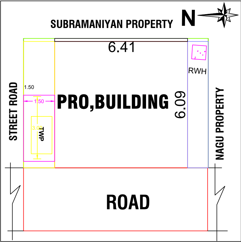
SITE PLAN
