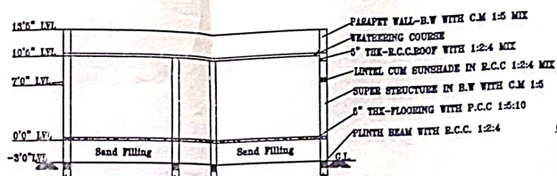
SECTION THROUGH A-B
