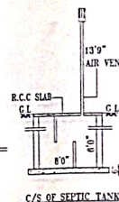
C/S OF SEPTIC TANK
