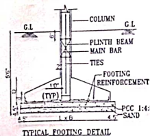
TYPICAL FOOTING DETAIL
