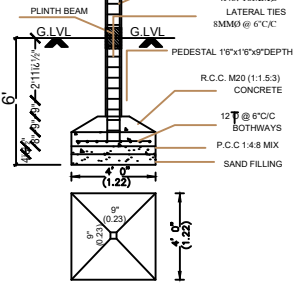
FOUNDATION DETAIL
