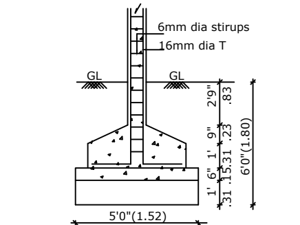
COLUMN FOUNDATION DETAIL
