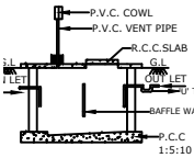
SEC. OF SEPTIC TANK
