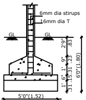
COLUMN FOUNDATION DETAIL
