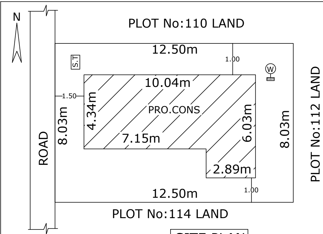
SITE PLAN
