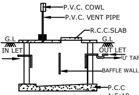
SEC. OF SEPTIC TANK
