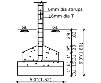
COLUMN FOUNDATION DETAIL
