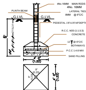
FOUNDATION DETAIL
