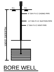
BORE WELL
