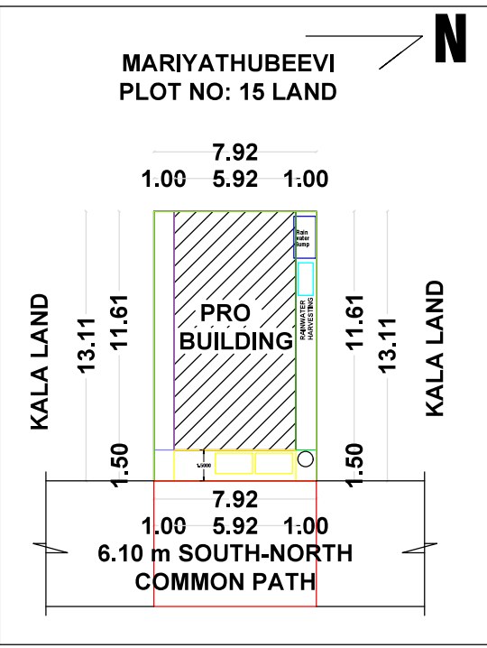
SITE PLAN & KEY PLAN (1:100)
