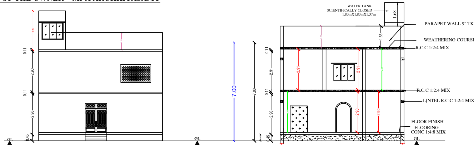
FRONT ELEVATION
