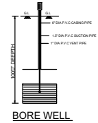
BORE WELL
