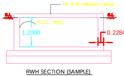
RWH_CAPACITY_L=2000LTRS
