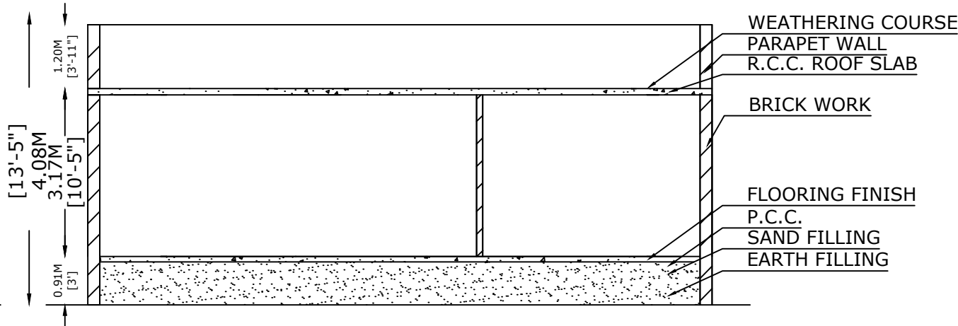
SECTION AN AA
