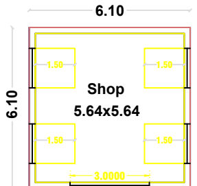
PRO. GROUND FLOOR PLAN
