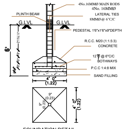
FOUNDATION DETAIL
