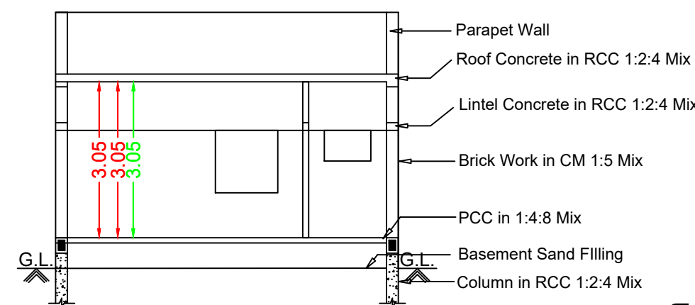
Section RR
