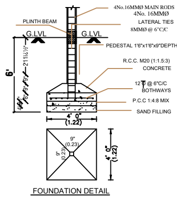
FOUNDATION DETAIL
