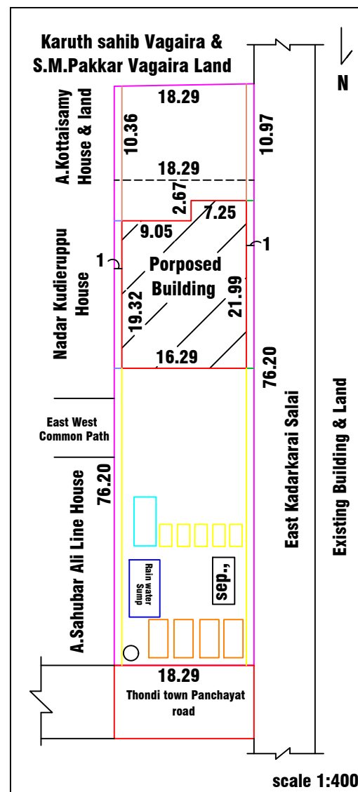
SITE PLAN CUM KEYPLAN
