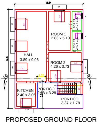
PROPOSED GROUND FLOOR
