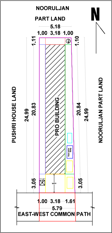
SITE PLAN & KEY PLAN
