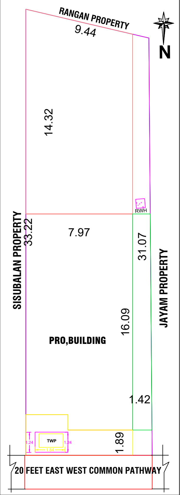
SITE PLAN
