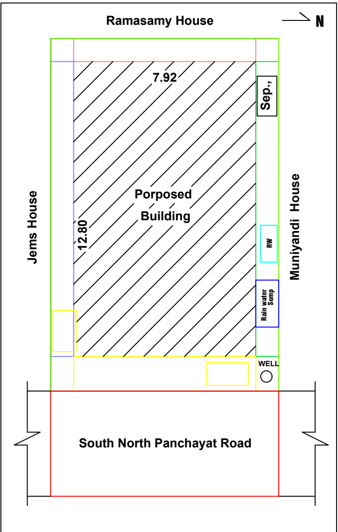
SITE PLAN CUM KEYPLAN
