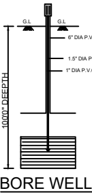
BORE WELL
