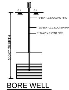
BORE WELL
