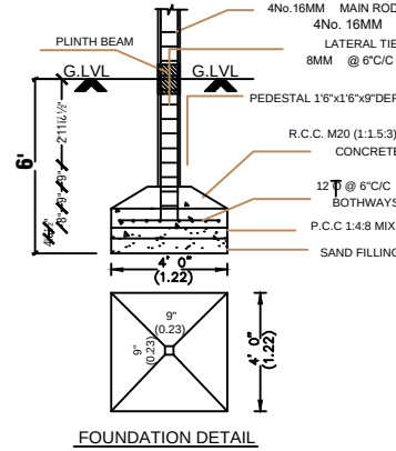
FOUNDATION DETAIL
