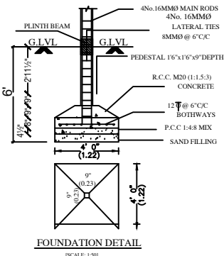
FOUNDATION DETAIL
