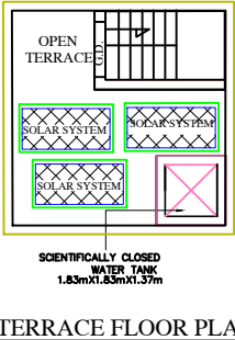
TERRACE FLOOR PLAN
