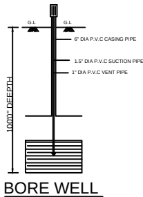
BORE WELL
