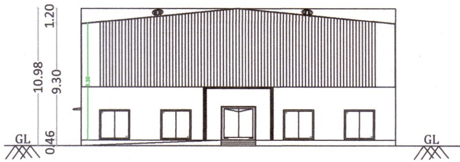
ELEVATION SCALE 1:100
