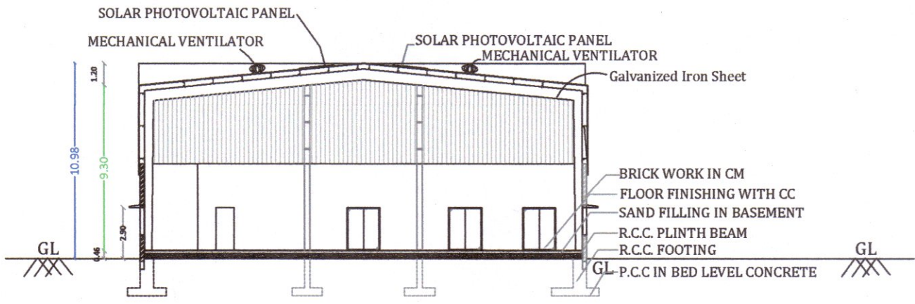
SECTION-AA SCALE 1:100
