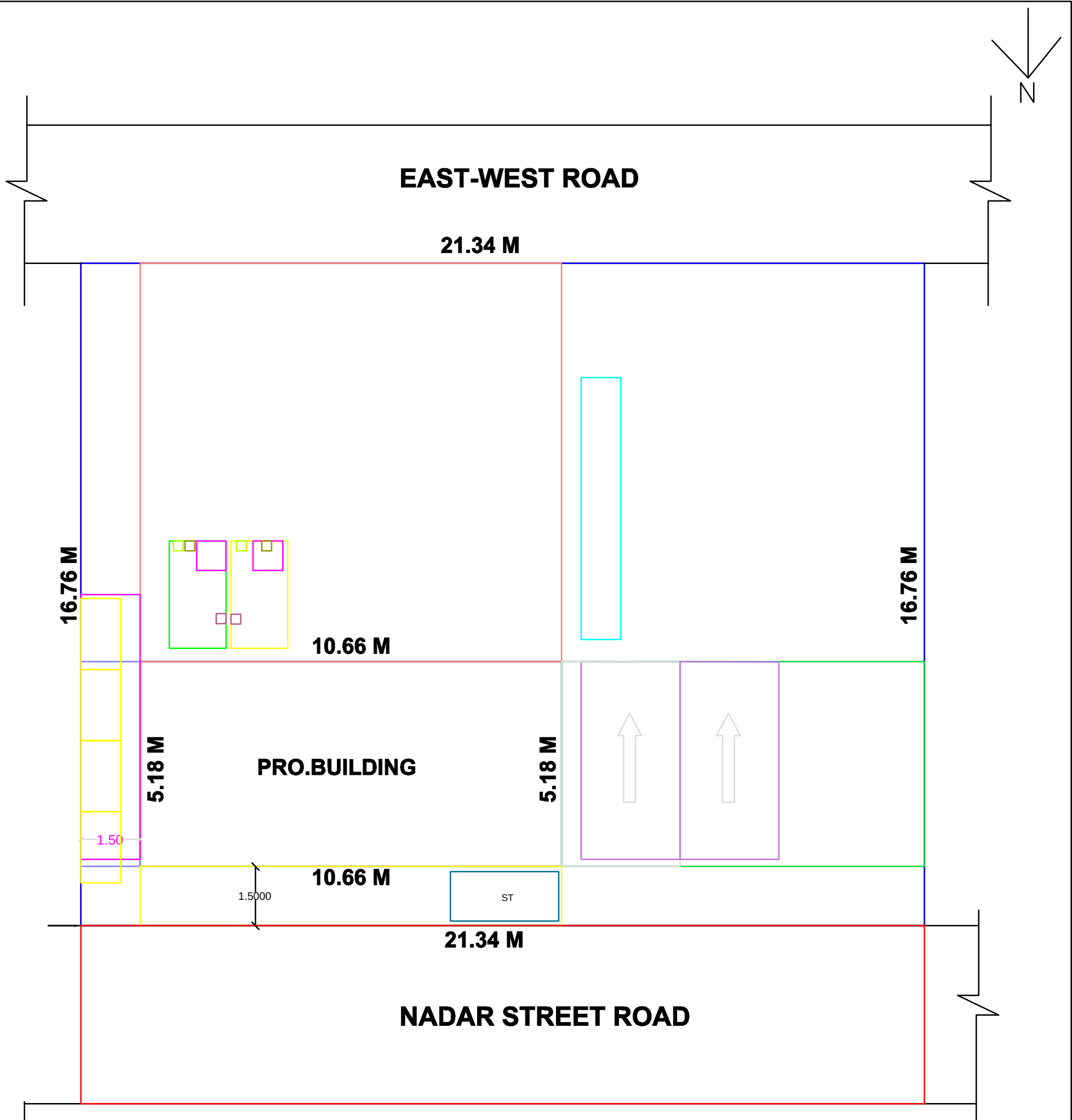
SITE FLOOR PLAN PROPOSED
