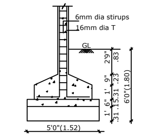
COLUMN FOUNDATION DETAIL
