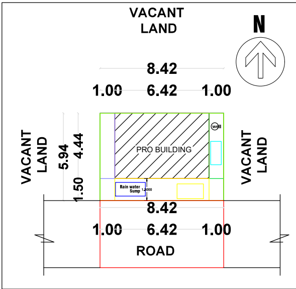
SITE PLAN & KEY PLAN
