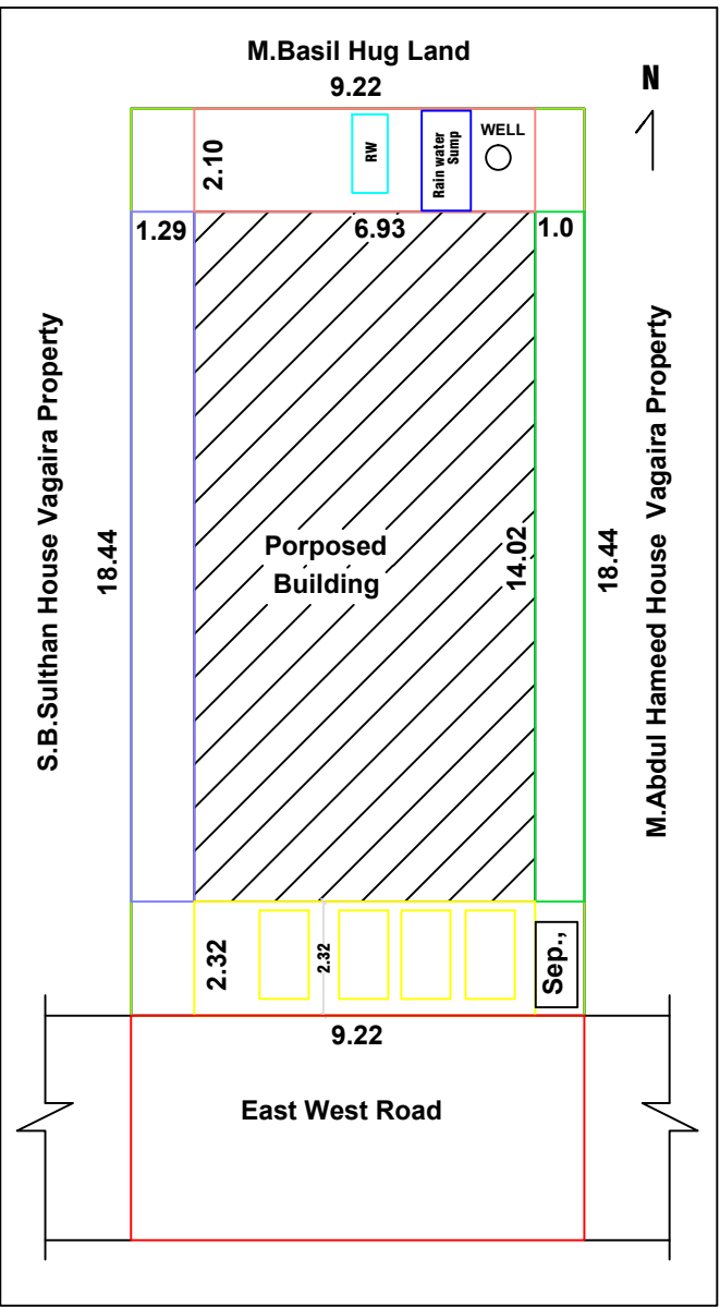
SITE PLAN CUM KEYPLAN
