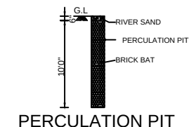
PERCOLATION PIT
