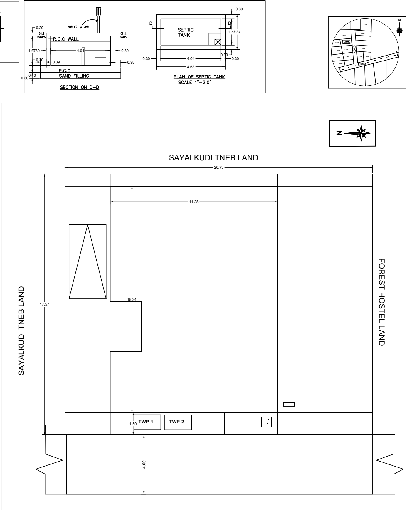
SITE PLAN
