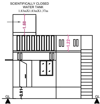
FRONT ELEVATION
