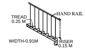
STAIRCASE DETAILS
