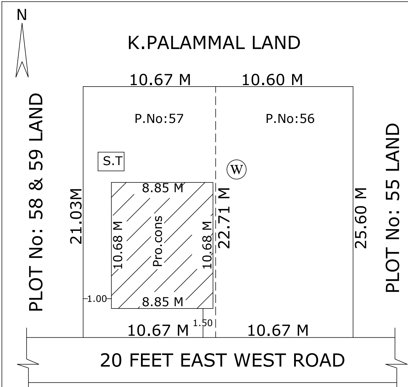
SITE PLAN
