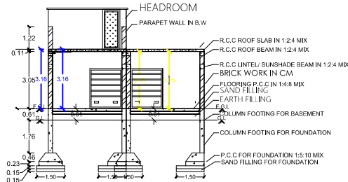
SECTION ON-A-A
