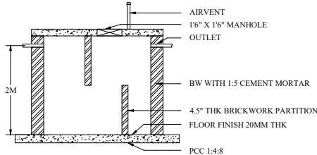
CROSS SECTION OF SEPTIC TANK
