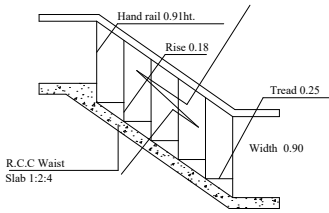
STAIRCASE DETAIL
