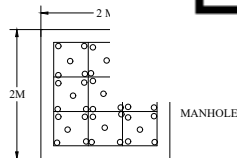
PLAN OF RAIN WATER RECHARGING PIT
