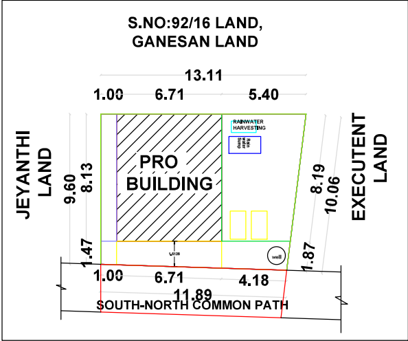
SITE PLAN & KEY PLAN (1:100)
