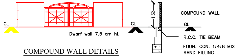
SECTION
