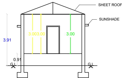
SECTION ON-AB
