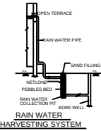
RAIN WATER HARVESTING SYSTEM
