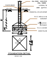
FOUNDATION DETAIL
